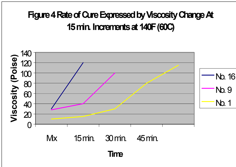
FIGURE IV Rate of Cure Expressed by Viscosity Change @15 minute Increments at 140°F (60°C)
