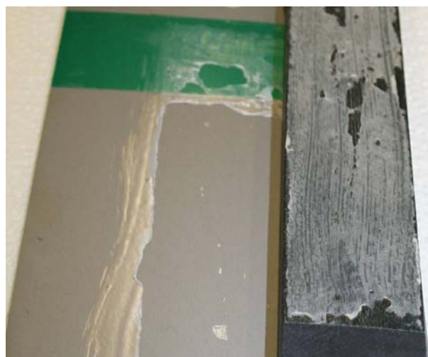
Figure 10. Total adhesive failure of 3M-30NF to steel.
