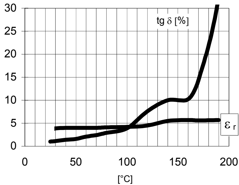
Loss factor ( \tan \delta ) and dielectric constant ( \epsilon_r ) as a function of temperature (measurement frequency: 50 Hz / IEC 60250)
