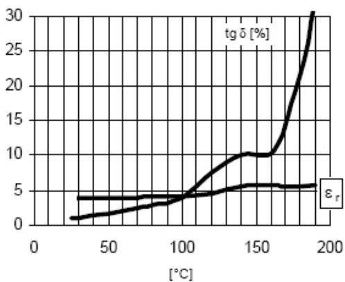
Fig. 7.1 Loss factor ( \tan \delta ) and dielectric constant ( \epsilon_r ) as a function of a function of temperature System A: 64% filler content
