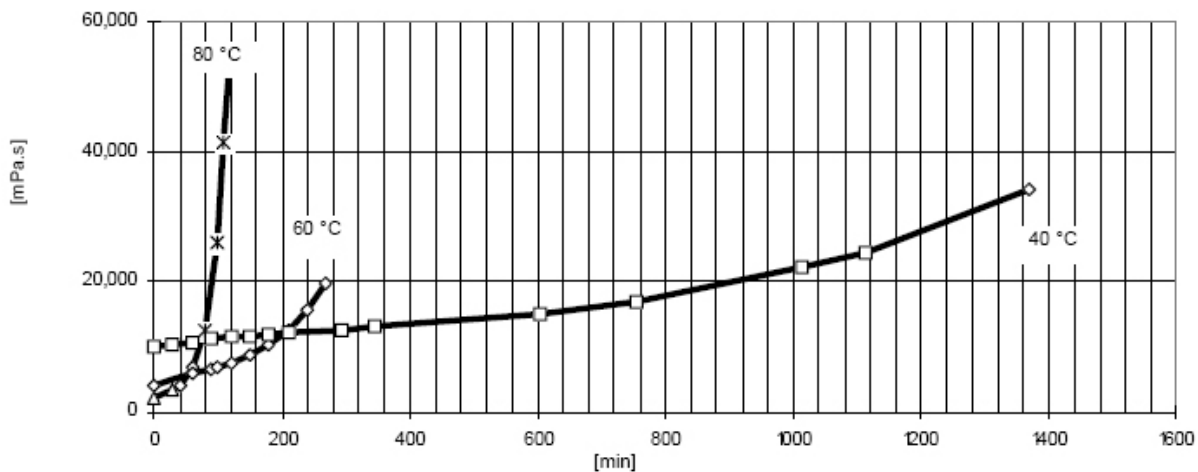
Fig. 5.1 Viscosity increase at 40°C, 60°C and 80°C*: System A: 64% filler content
