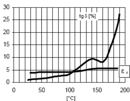
Fig. 7.2 Loss factor ( \tan \delta ) and dielectric constant ( \epsilon_r ) as a function of a function of temperature System B: 66% filler content
