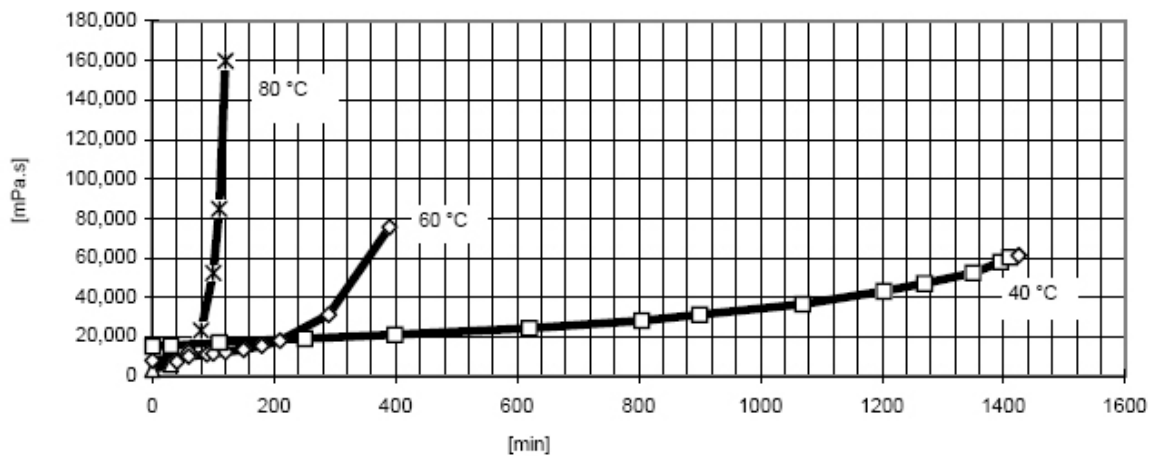
Fig. 5.2 Viscosity increase at 40°C, 60°C and 80°C*: System B: 66% filler content
